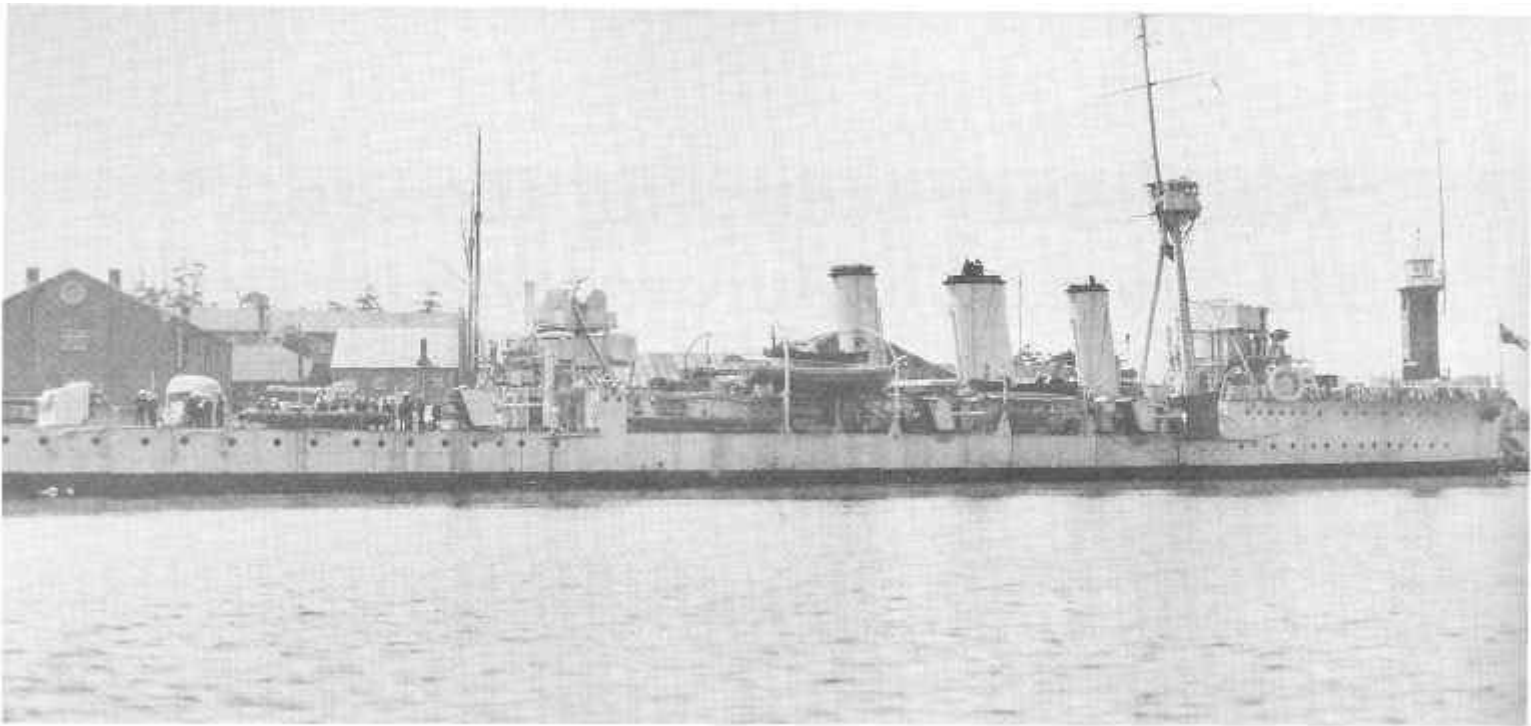
Aurora in profile, April 1921. The arrangement of the armament is clearly seen: 6-inch guns immediately forward and aft, with three 4-inch guns on either broadside. The gun without a shield forward of the after 6-inch gun is the 4-inch HA. Between the two is a dome-shaped structure, probably a shelter for the gun crews. The starboard torpedo tubes are the dark objects, one pair beside the 4-inch HA, the other abaft the davits. When examined under magnification, this photo also shows the after visual range dial mounted below the rangefinder on the platform, between the curved searchlight control positions. Two men are working on top of the centre funnel.
