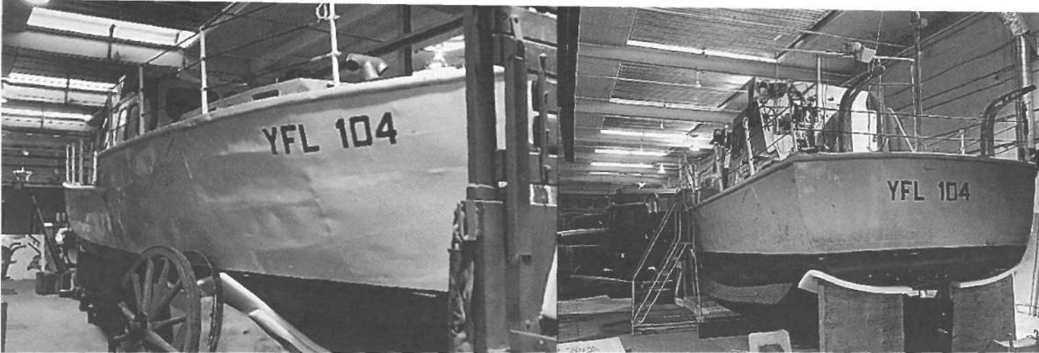
Left: Pogo's starboard side as seen from the objects and conservation workshop. The Naval designation "Yard Ferry Light -104" is clearly marked on her well used hull. Right: Stern view of Pogo on her temporary cradle at Vimy House, the Canadian War Museum's storage facility. (Photos by Bill Kent, CWM Collection)
